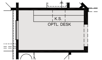
OPTIONAL COMPUTER AREA #3 10'-5" X 6'-4"
