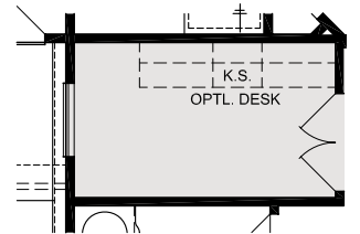
OPTIONAL COMPUTER AREA #2 10'-8" X 6'-4"
