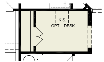
OPTIONAL COMPUTER AREA #1 8'-1" X 6'-4"
